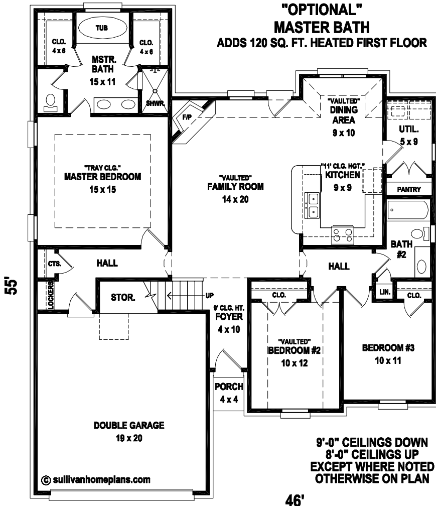
FIRST LEVEL FLOOR PLAN
