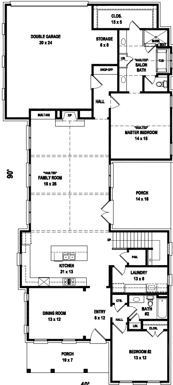
FIRST LEVEL FLOOR PLAN
